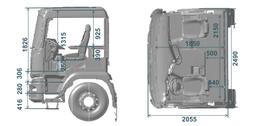
• Medium-length flat-roof wide-body cab
